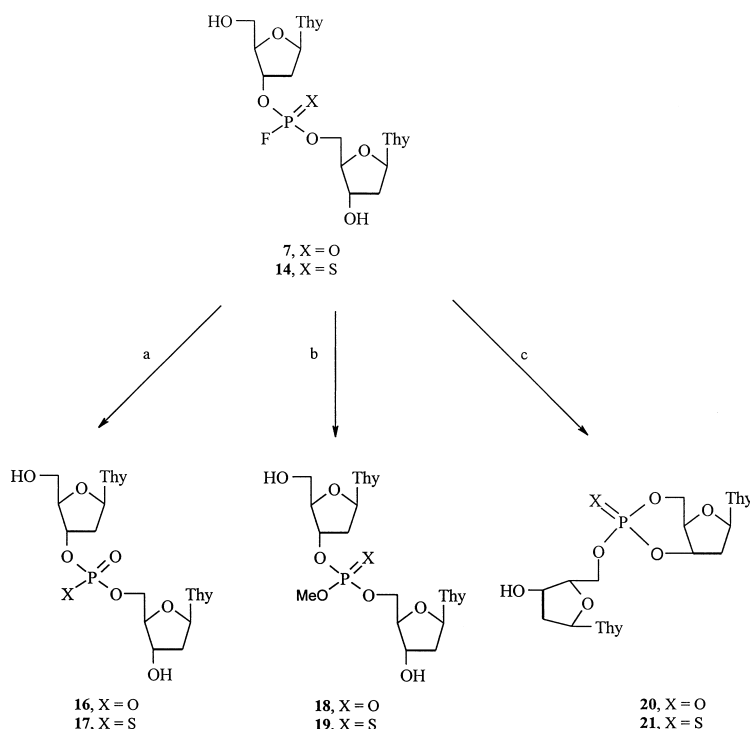
Scheme 3. (a) Tris–HCl pH8 or \text{NH}_4\text{OH} ; (b) MeOH, \text{Et}_3\text{N} ; (c) DBU.
