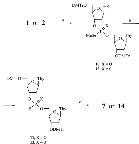
Scheme 2. (a) (i) 3'- O -DMTr-thymidine, DBU; (ii) MeI; (b) AgF for 10 , \text{Et}_3\text{NHf} for 12 ; (c) p -toluenesulfonic acid.
